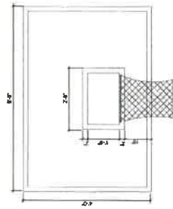
BLACKBOARD (FRONT VIEW) SCALE: 3/4" = 1'-0"
