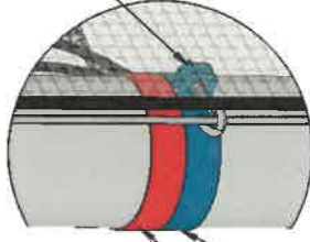
DETAIL C
