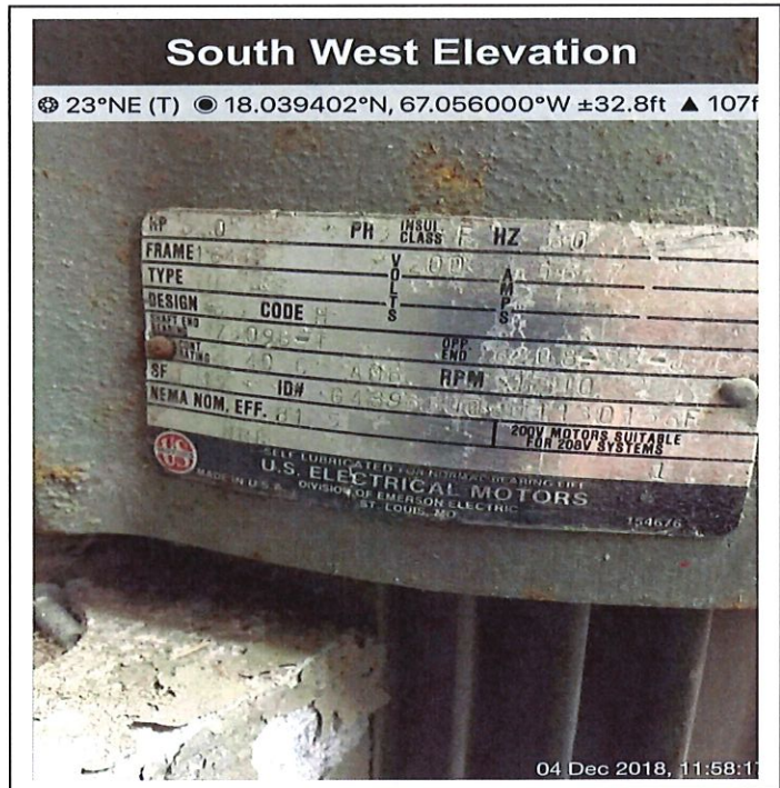
Lajas (CDT) water pump motor tag-pump 2
