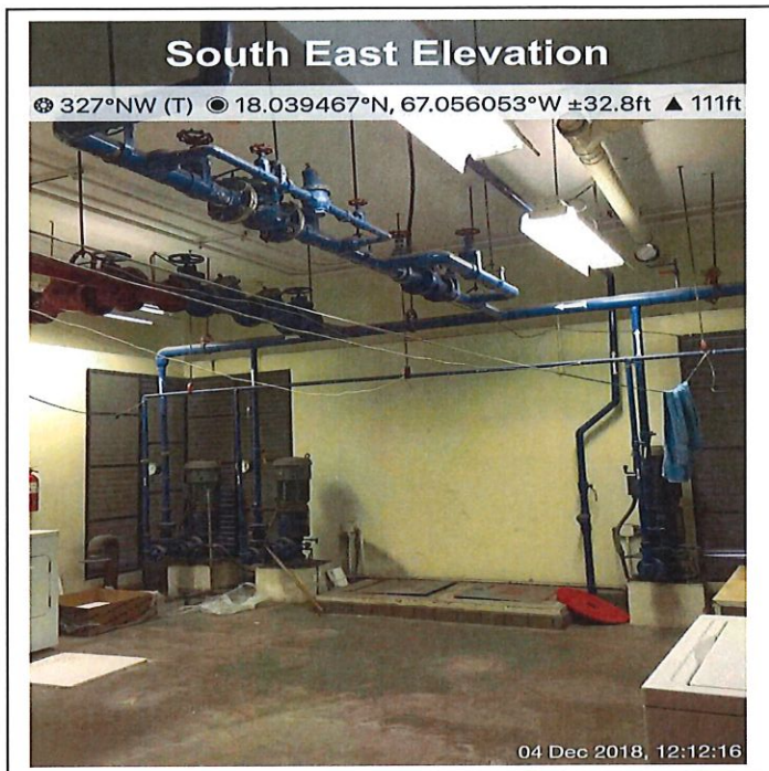
Lajas (CDT) water pump and ground tank room
