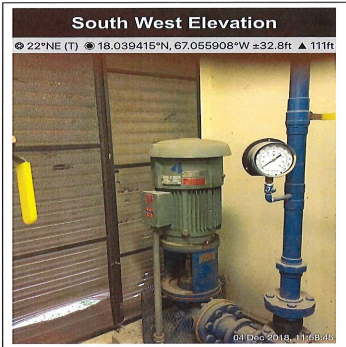
Lajas (CDT) 3-phase water pump motor-pump 4
