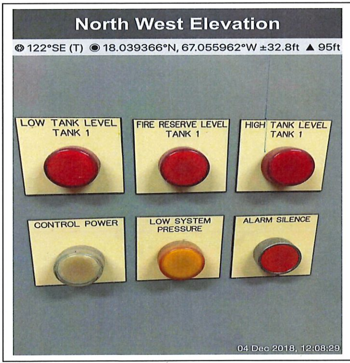
Lajas (CDT) water pump control panel
