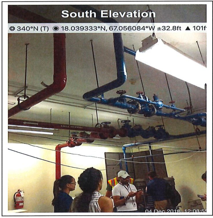
Lajas (CDT) fire and local water supply line, single access point
