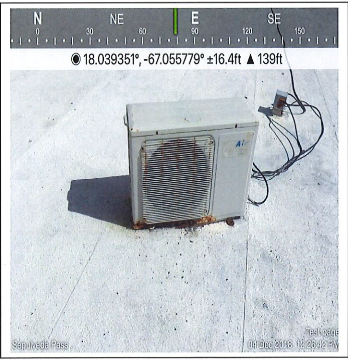
Lajas (CDT) roof a/c split condensing unit, 9000 BTU, for IT server room
