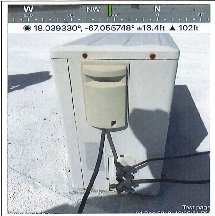
Lajas (CDT) roof a/c split condensing unit, 9000 BTU, for IT server room
