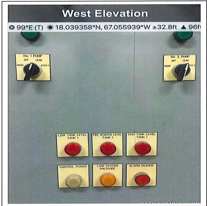
Lajas (CDT) water pump control panel
