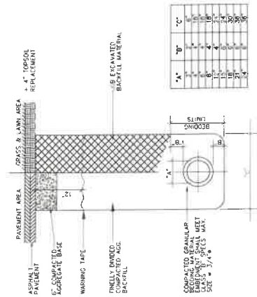
TRENCH AND BACKFILL DETAIL
