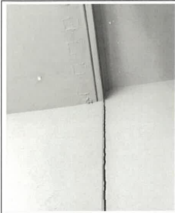
2nd Floor Middle Exterior Stairwell – Detachment of Elevator Shaft Structure From Exterior Stairwell Shown
